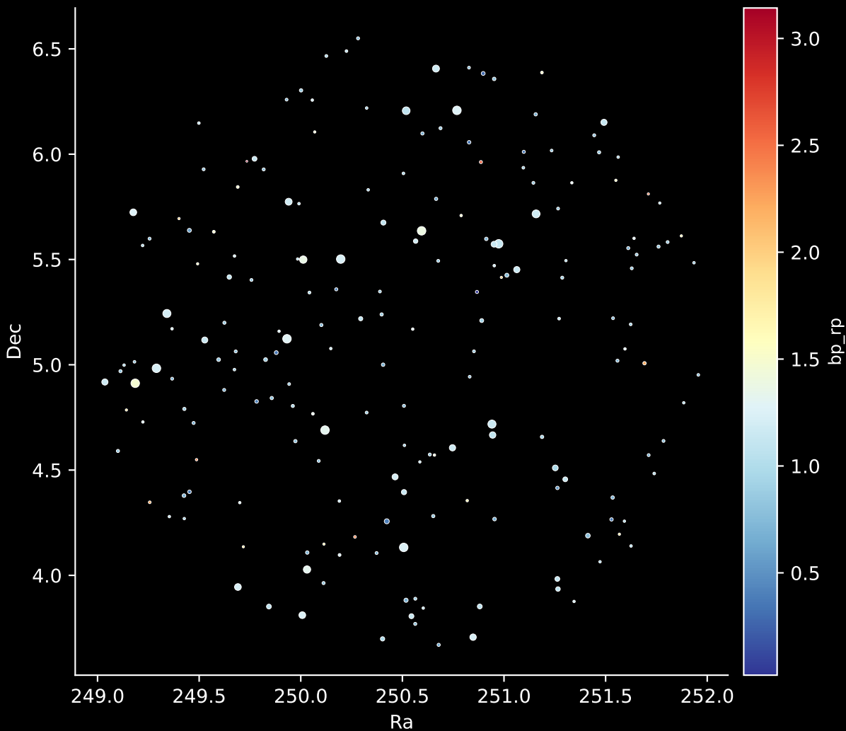
APOGEE DR17 Field: [234+44_MGA] Stars: 194
