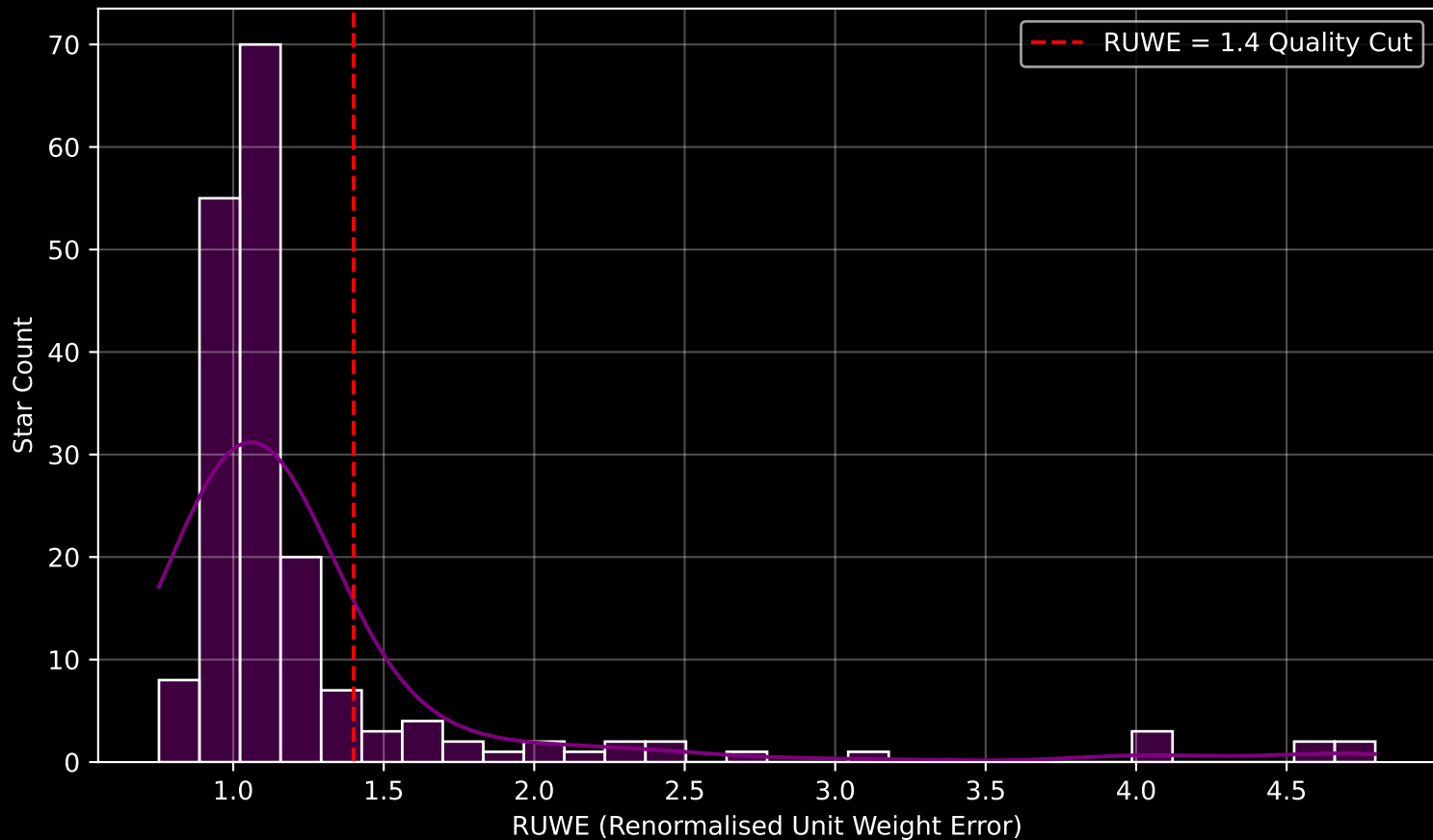
GAPOGEE DR17 Field [234+44_MGA] RUWE Distribution (n= 186)
