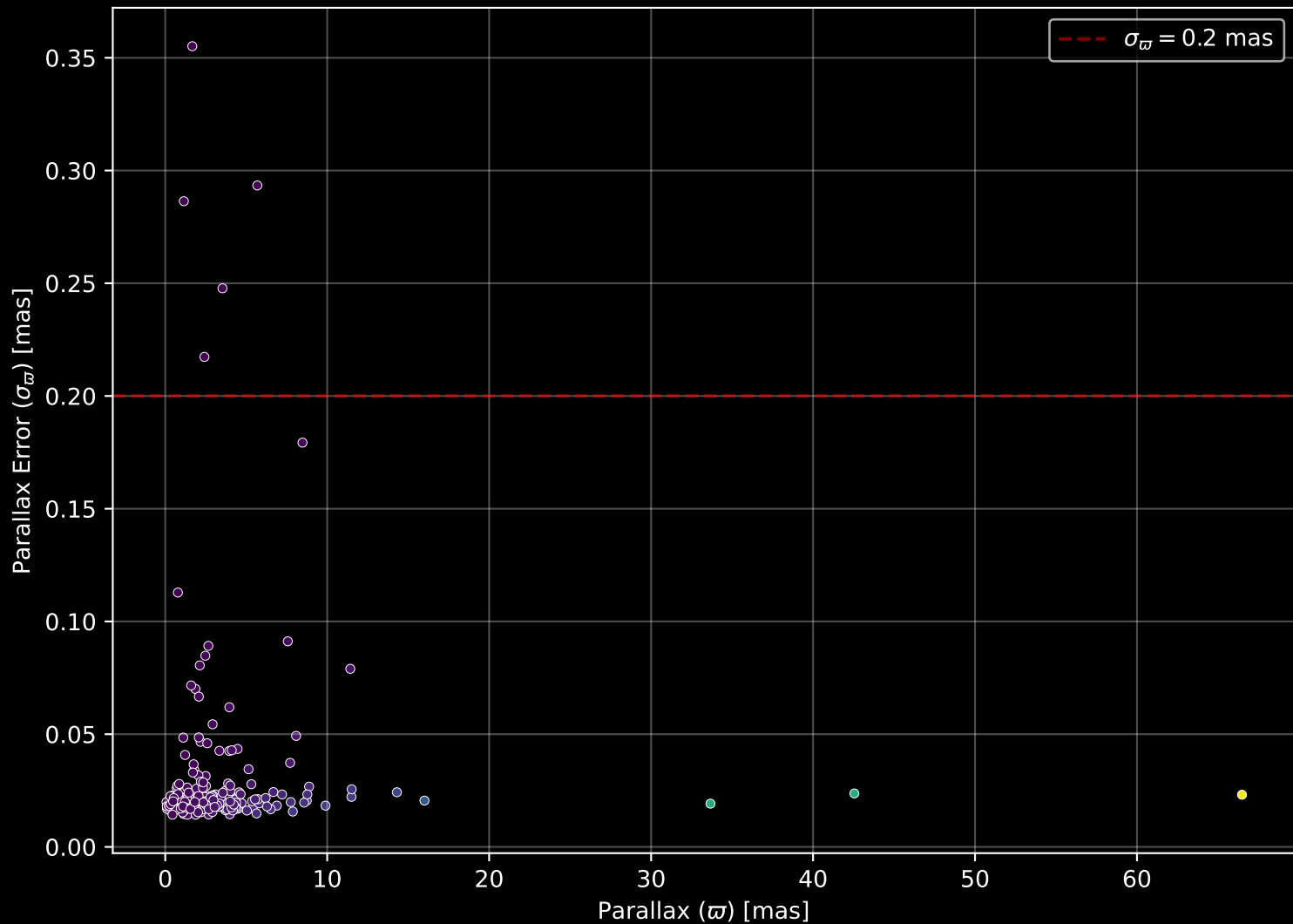
APOGEE DR17 Field: [234+44_MGA] Parallax Quality (n= 194)
