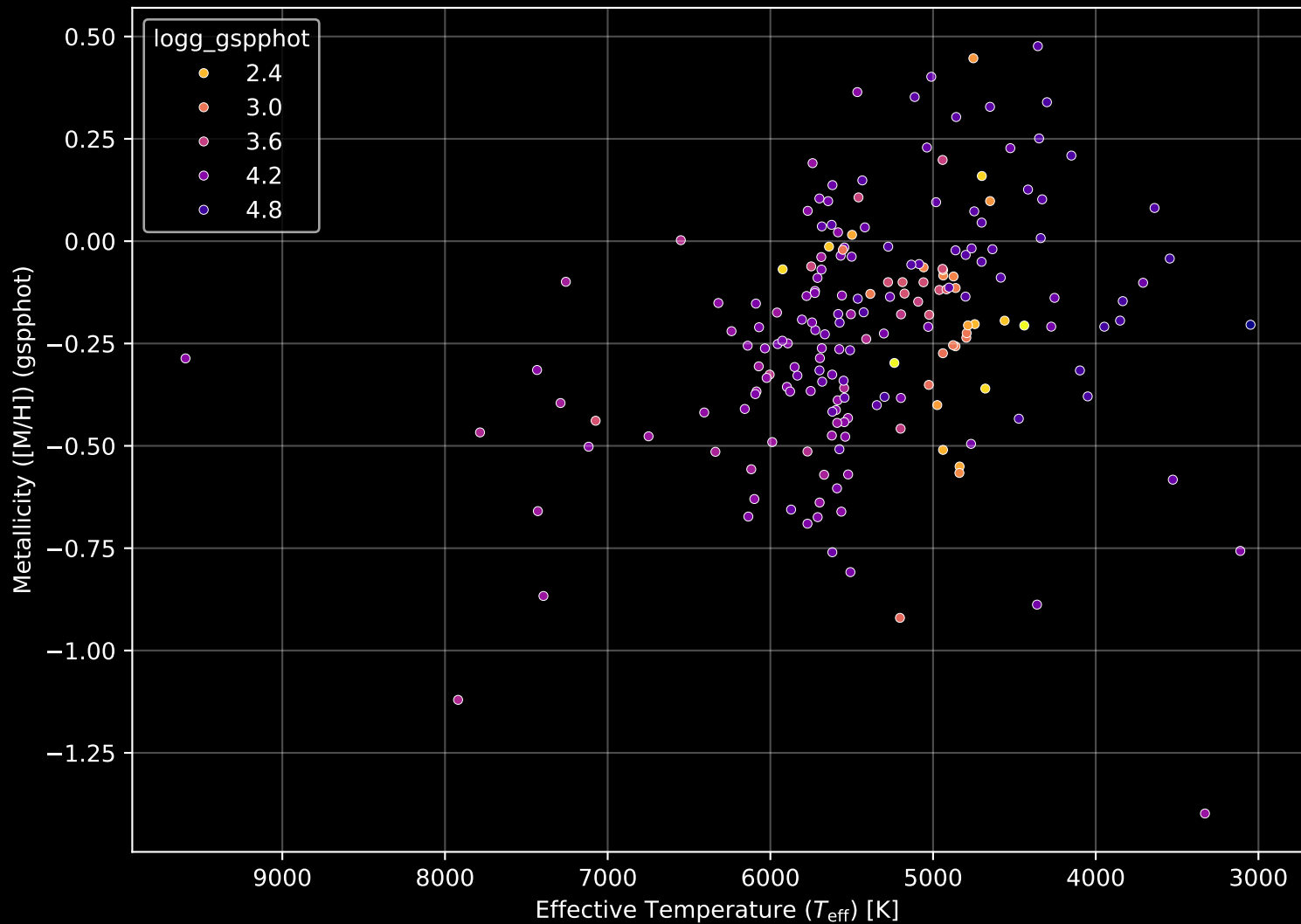
APOGEE DR17 Field: [234+44_MGA] Stellar Population Parameters (n= 194)
