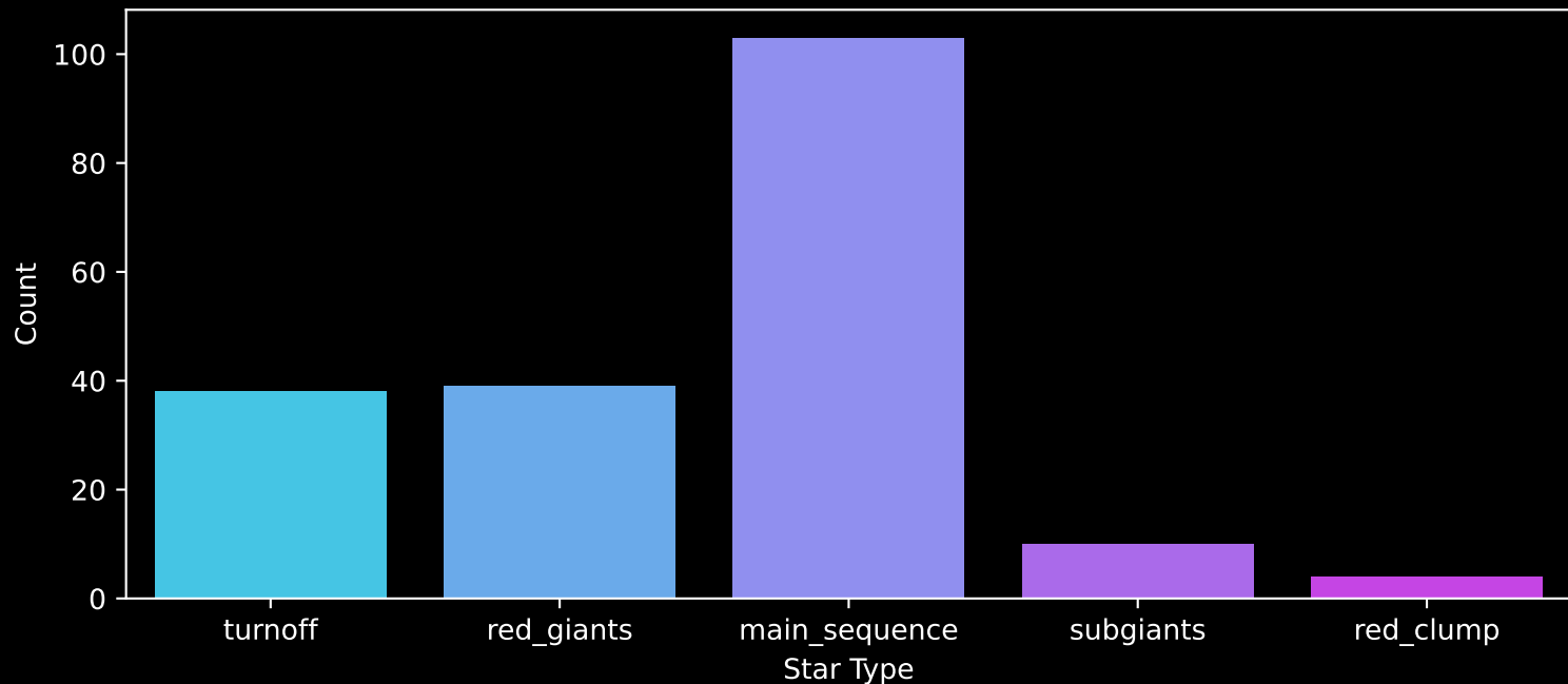
APOGEE DR17 Field: [234+44_MGA] Count plot of Star Type
