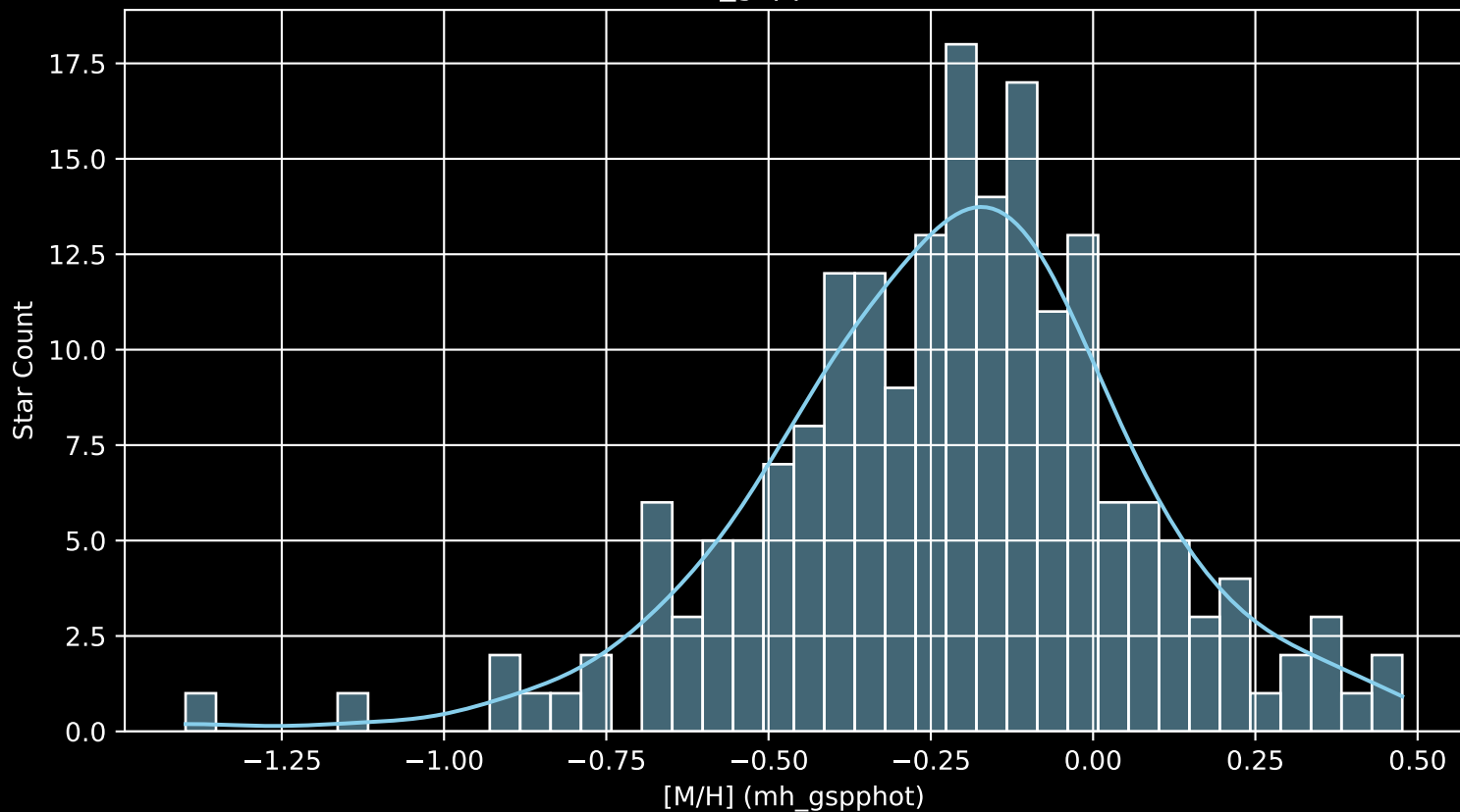
APOGEE DR17 Field: [234+44_MGA [M/H] (mh_gspphot) (n= 194)
