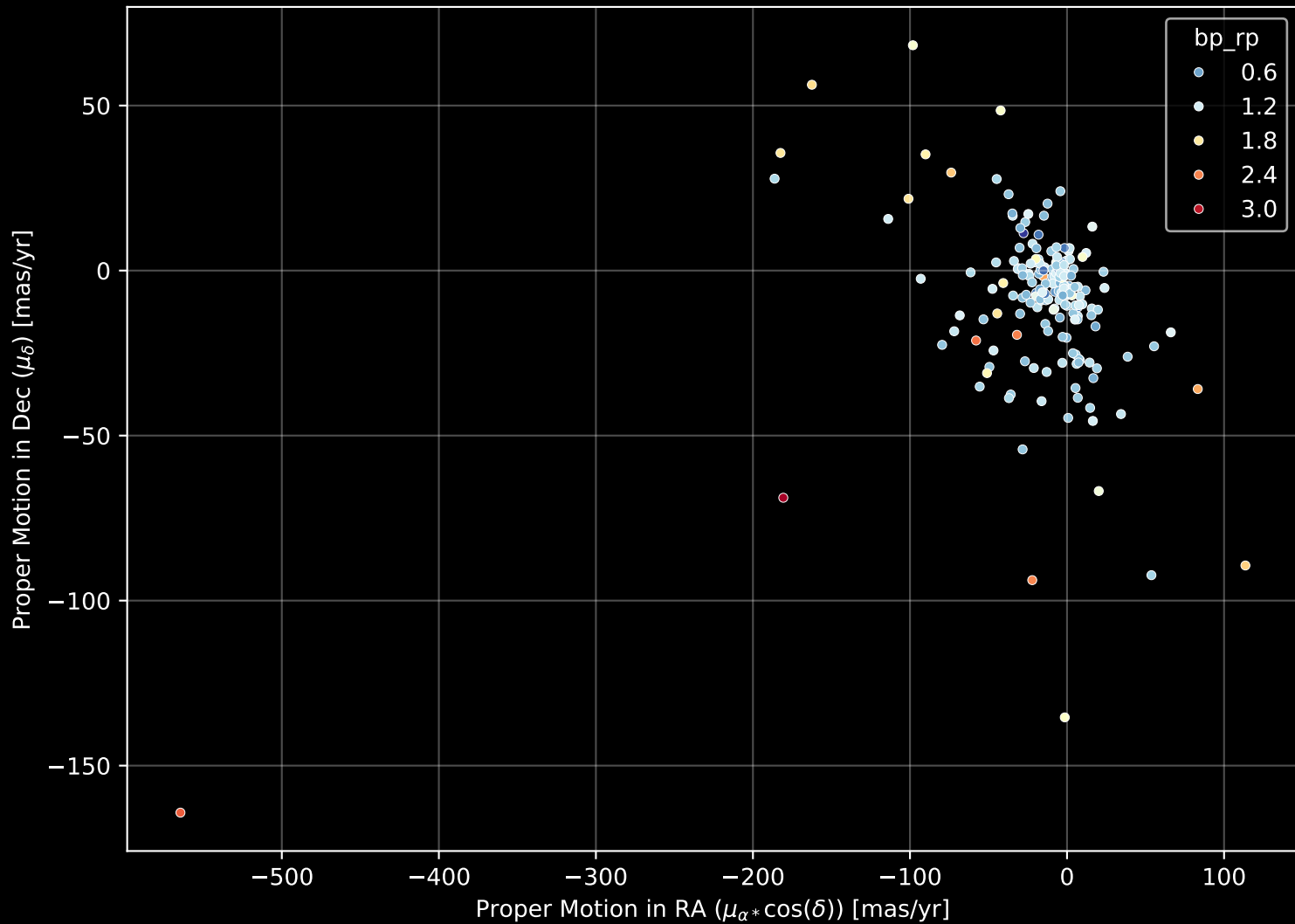
APOGEE DR17 Field: [234+44_MGA] Proper Motion Diagram (n= 194)
